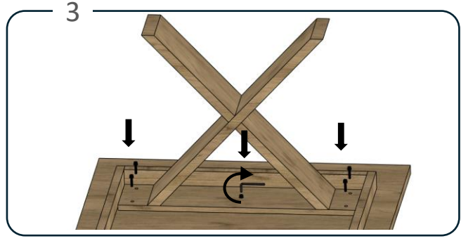
Use the Allen key with to fix the legs to the top by turning the bolts with washers into the pre-drilled holes in the leg supports.
