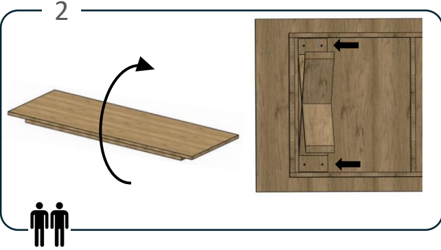
Turn the table top upside down and place legs on both ends of the frame to match the pre-drilled holes in the top and leg supports.
